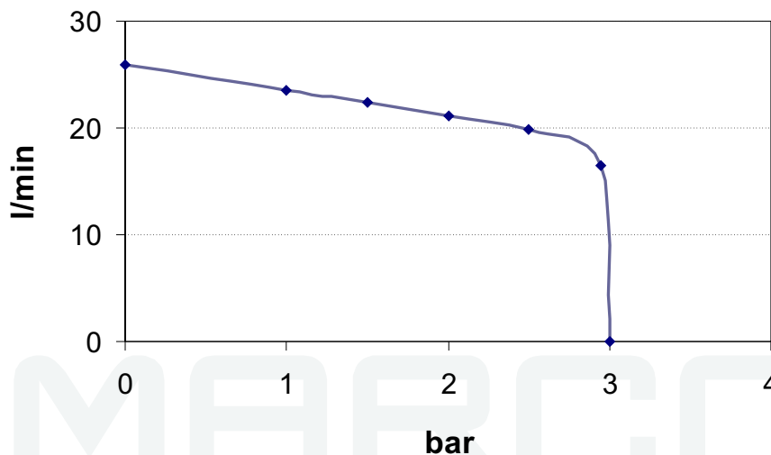
DIAGRAMMA PORTATA FLOW RATE DIAGRAM
